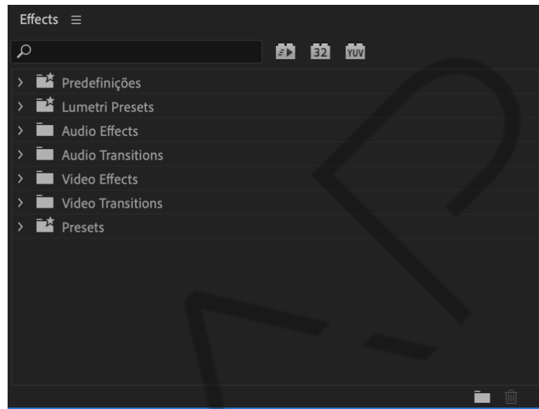
Figura 21 – Janela Effects
